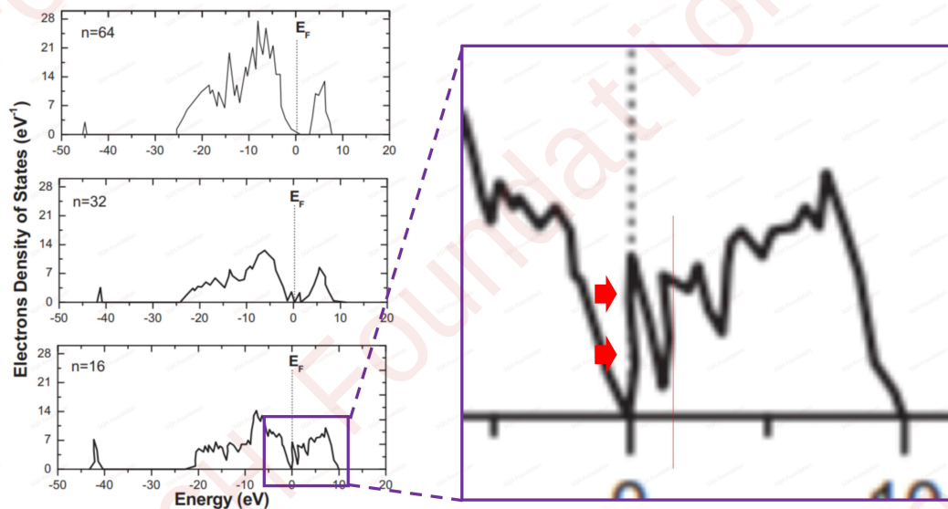
Fig. 2. TDOS of B-doped diamond films. Here n is the total number of C-atoms along with one boron atom in each cell.
